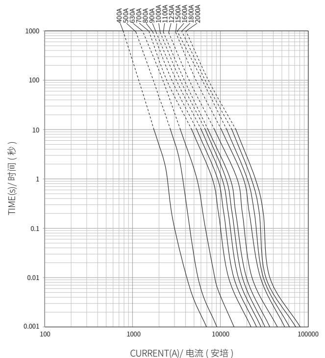
H4FGaBat 平均 I-T 曲线图 (仅供参考) AVERAGE I-T CHARACTERISTICS CURVE (FOR REFERENCE ONLY)
